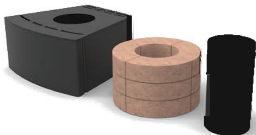
The heat storage kit includes the stove extension, heat storage bricks and pipe extension
