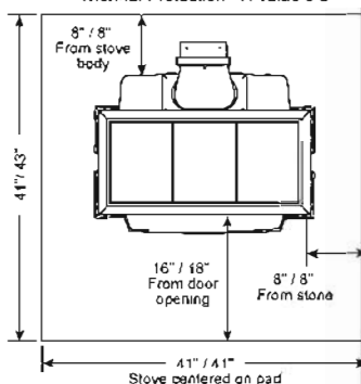
Minimum Hearth Protection US/Canada: Thermal Protection R-value 6.6
