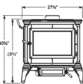
Shown with optional ash pan
