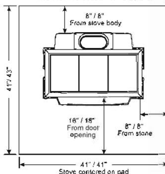
Minimum Hearth Protection US/Canada: Thermal Protection R-value 2.5
