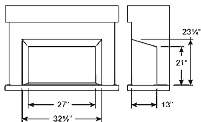
Minimum Fireplace Opening:
